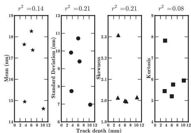
Fig. 7. The moments of the droplet diameter size distribution (not corrected for completeness and projection) as a function of depth along Stardust aerogel debris Track 35. The Pearson coefficient of determination ( r^2 ) for the correlation of the moments with track depth is given above the plot.
